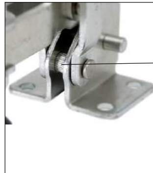
Hardened Bushes
