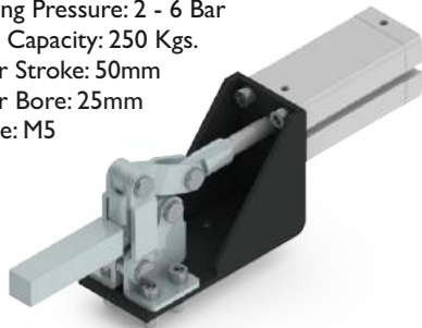
Clamp Arm Opening: 90°
