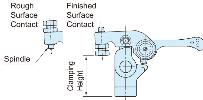
Clamping Position
