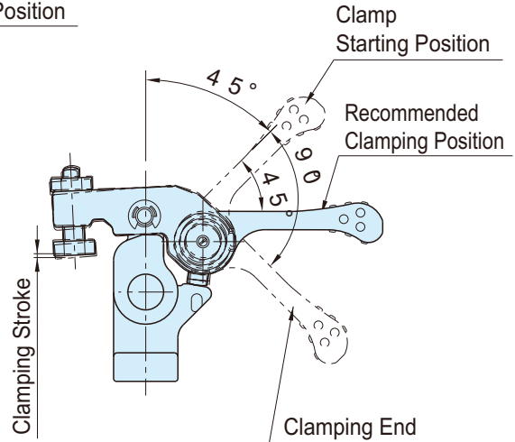
Clamping Throw
